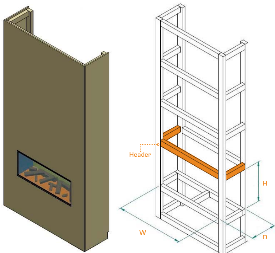
New Forest 1900 mm Open Dimensions
