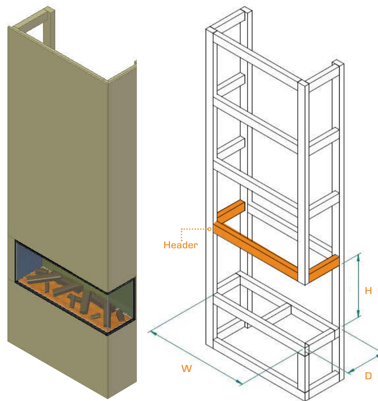
New Forest 1900 mm Open Dimensions
